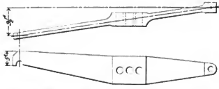
Figs. 1668-1669. Trailing Truck Equalizer for Atlantic (4-4-2) Locomotive. American Locomotive Co.
